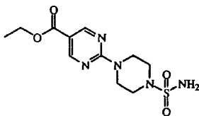
intermediate 10
